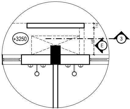
DETAIL- A (SCALE 1:25)
