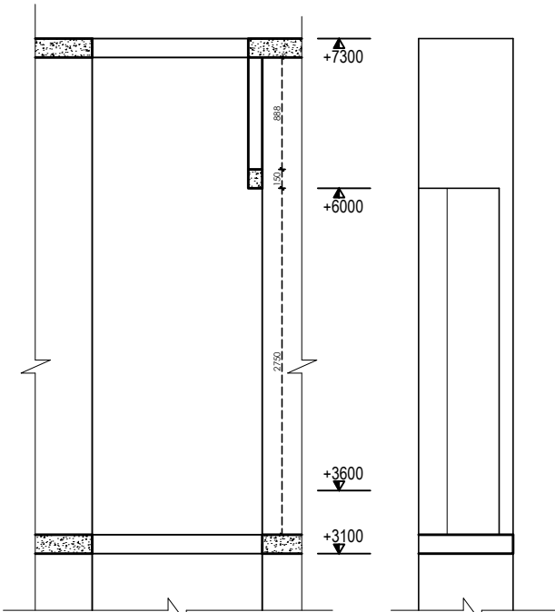
SECTION-3 (SCALE 1:25)
